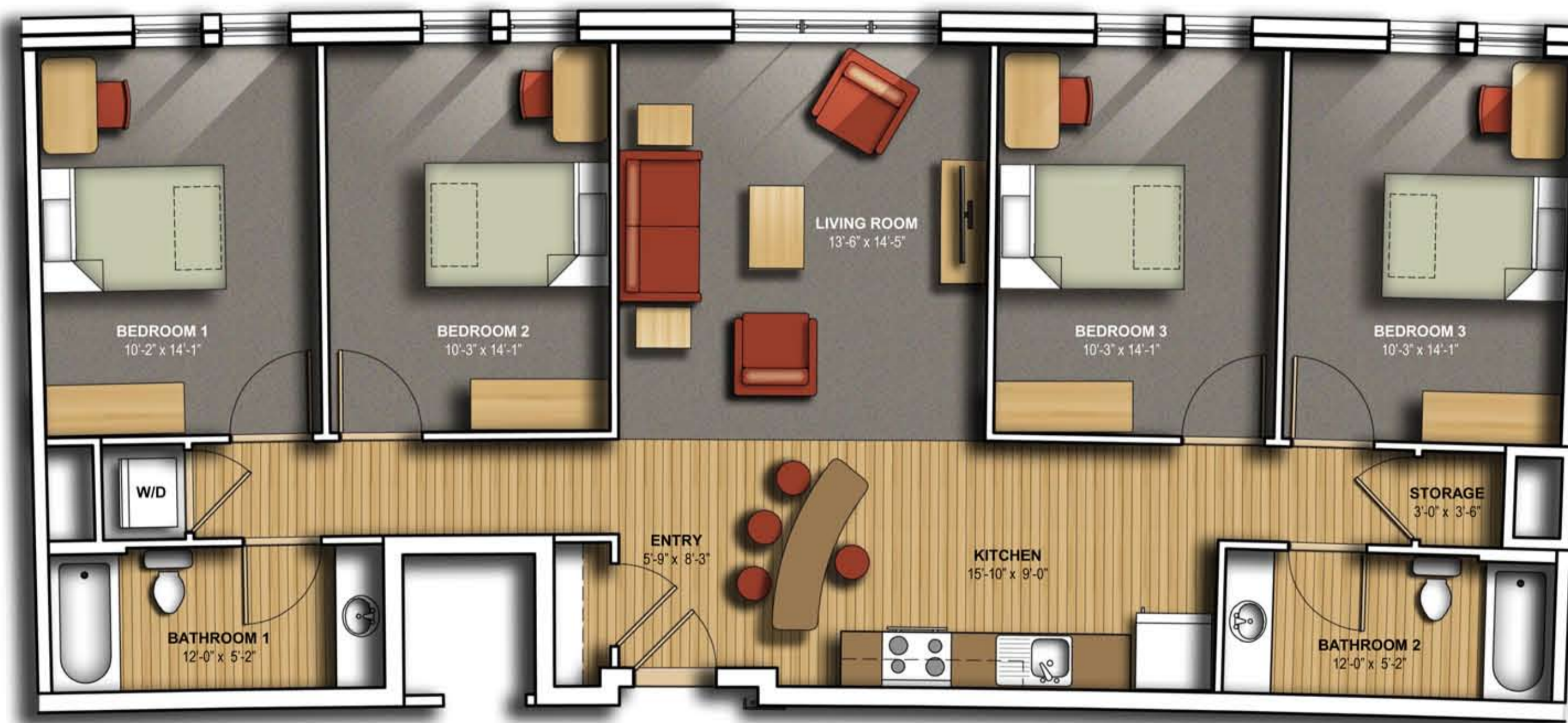
TYPICAL 4-BEDROOM MID-UNIT
